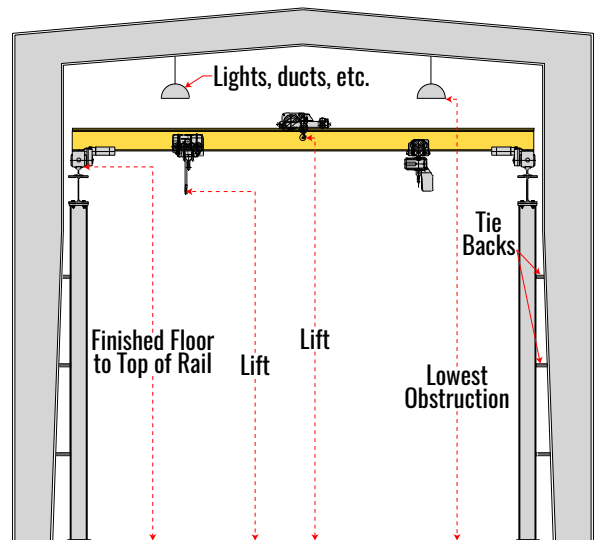
Crane Tie Back
