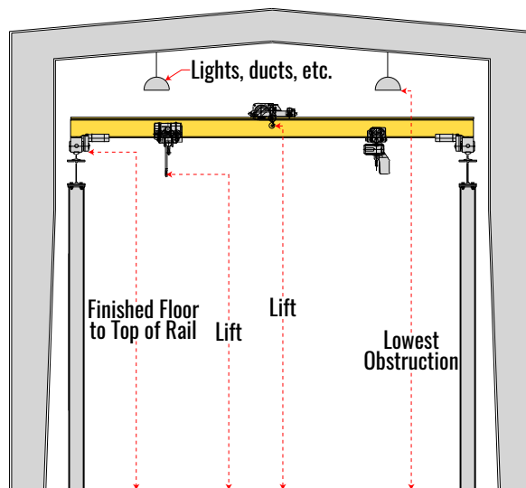
Free Standing Crane
