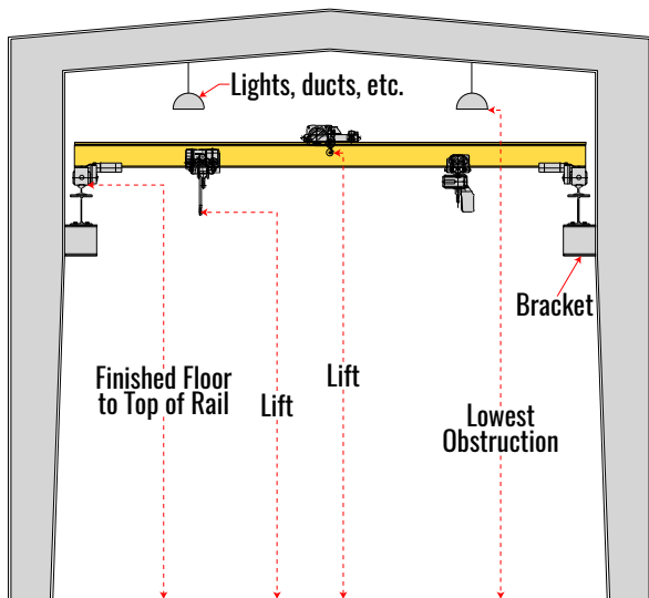
Crane Column Bracket
