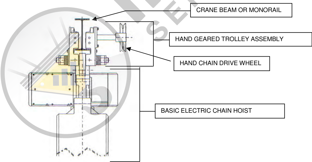
Figure 3. Hand Geared Trolley
