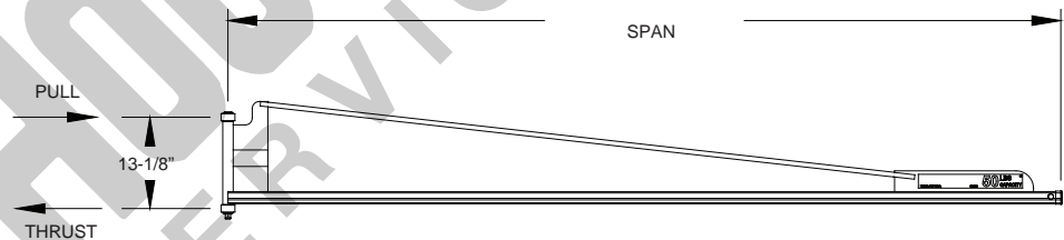
Diagram 1A. Wall/Column Mounted Tool Solutions Jib.
