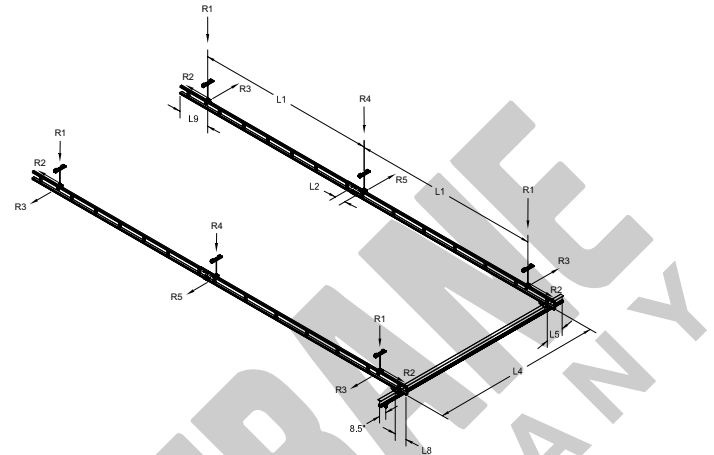
Diagram 2. Applied forces from bridge to supporting structure.
