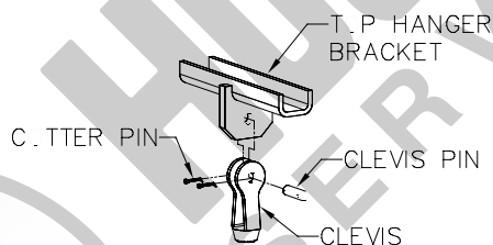
Diagram 2B. Attaching clevis to top hanger bracket.
