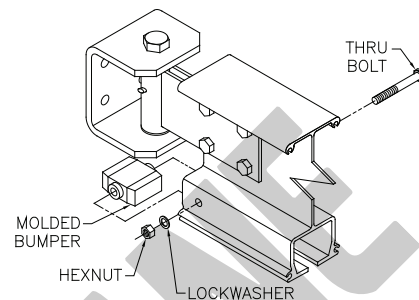
Diagram 3A. Endstop installation.
