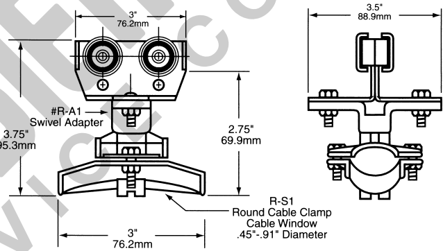
TROLLEY ASSEMBLY R-TR2A
