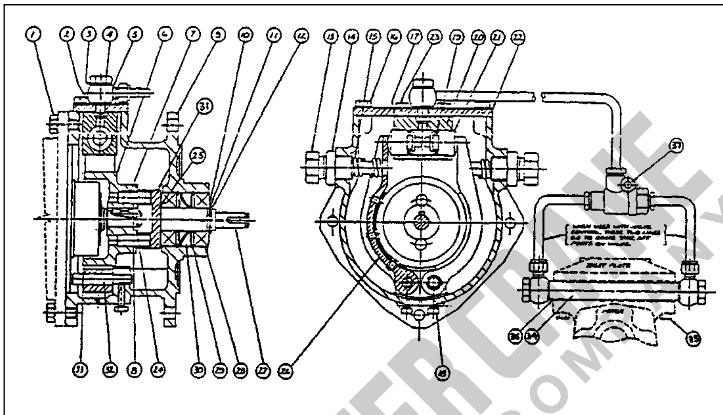
Figure 5. Brake Parts
