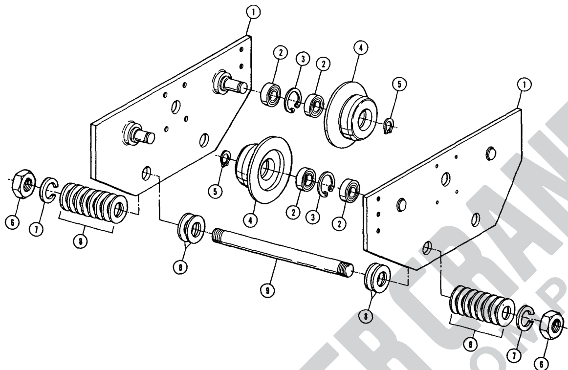
Figure 4. Push Type Rigid Mount Trolley Assembly. (4" \varnothing Wheels — 6" c/c Pins.)
