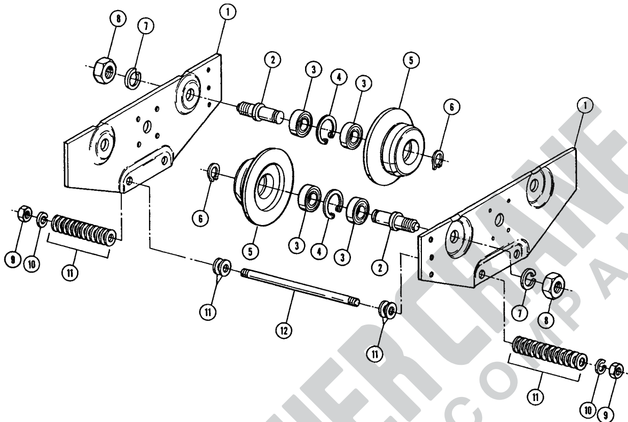
Figure 3. Push Type Rigid Mount Trolley Assembly. (4" \varnothing Wheels — 3-1/8" & 5" c/c Pins.)
